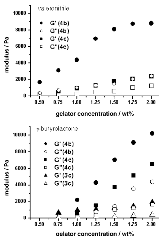
Figure 6. Influence of the concentration of the amide/urea-functionalized derivatives 4b (circles) and the 4c (squares) and bisamide 3c (triangle) in valeronitrile (top) and in \gamma -butyrolactone (bottom) on storage modulus G' (filled symbols) and on loss modulus G'' (open symbols) at a frequency of 1 Hz.
