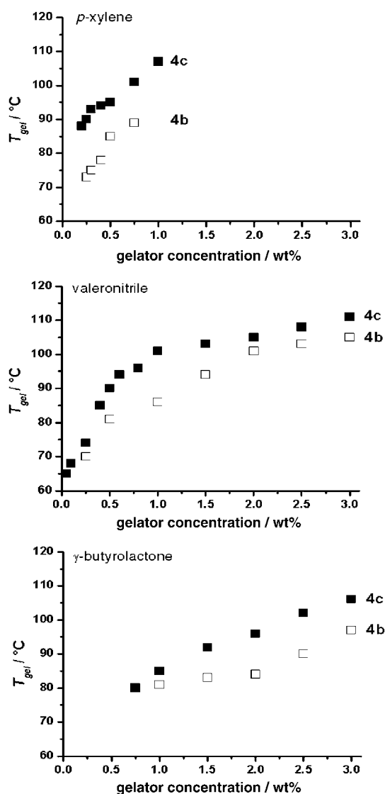
Figure 2. Sol–gel transition temperature as a function of the gelator concentration of compounds 4b (open squares) and 4c (filled squares) in p -xylene (top), valeronitrile (middle) and in \gamma -butyrolactone (bottom) determined by the dropping ball method.
