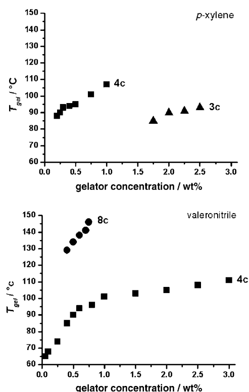
Figure 3. Sol–gel transition temperature as a function of the gelator concentration of bisamide 3c (triangles) and the amide/urea-derivative 4c (squares) in p -xylene (top) and of the amide/urea-derivative 4c (squares) and the bisurea derivative 8c (circles) in valeronitrile (bottom) determined by the dropping ball method.
