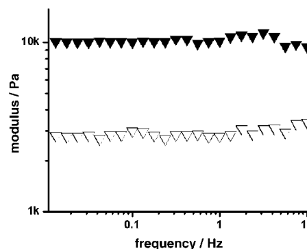
Figure 4. Dynamic rheological behavior of 4b in \gamma -butyrolactone at a concentration of 2 wt%. The plot shows the storage modulus G' (filled triangle) and loss modulus G'' (open triangle) versus frequency.
