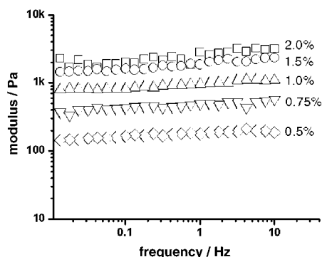
Figure 5. Comparison of the elastic storage modulus G' values versus frequency at different concentrations of gelator 4c in valeronitrile.
