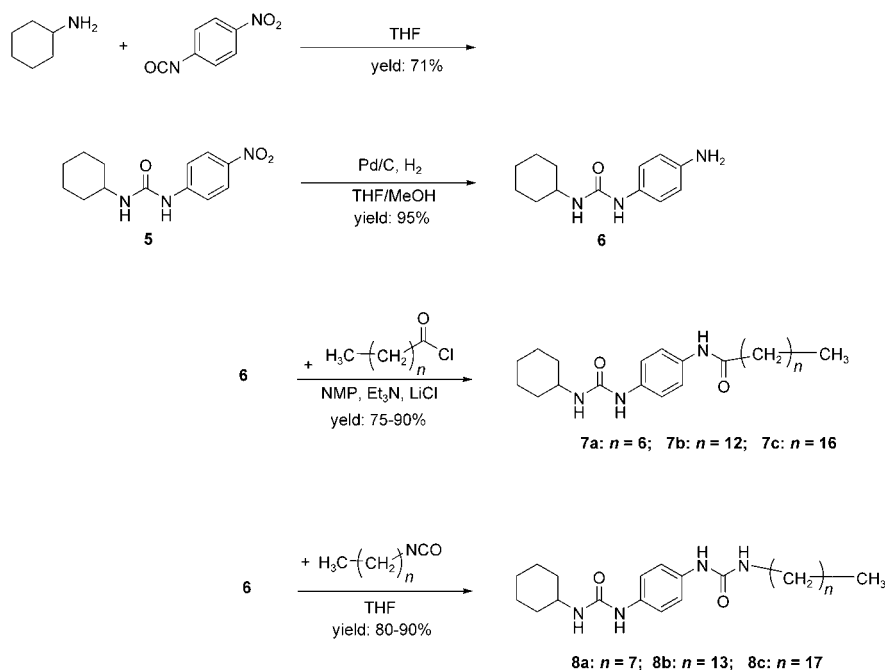
Scheme 2. Synthesis of asymmetrically substituted p -phenyldiamine-based urea/amide-functionalized derivatives 7a-c and bisurea derivatives 8a-c .
