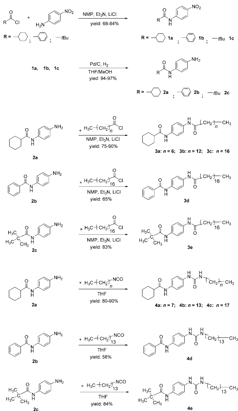
Scheme 1. Synthesis of asymmetrically substituted p -phenyldiamine-based bisamide derivatives 3a–e and amide/urea-functionalized derivatives 4a–e .
